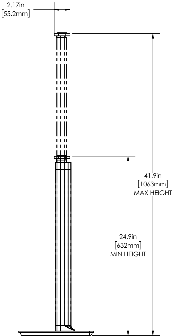
SIDE VIEW
